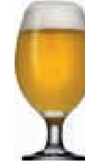
44417 BISTRO BİRA BEER v:~400 cc. 13 1/4 US oz. 14 UK oz. G*: 300 cc. h: 160 mm. 6 1/4" t: 68 mm. 2 3/4" b: 70 mm. 2 3/4" d: 86 mm. 3 1/2" SKU / PACKING 793616* fk12-2s/fb12-2s
