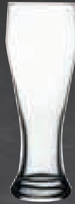
42126 WEIZENBEER & PILS BİRA BEER v:~520 cc. 17 1/4 USoz. 18 1/4 UK oz. G*: 400 cc. h: 217 mm. 8 1/2" t: 75 mm. 3" b: 70.5 mm. 2 3/4" d: 80.5 mm. 3 1/4" SKU / PACKING 747374* fk6-4s/fb6-4s
