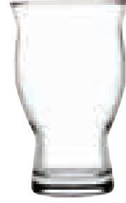
420108 REVIVAL BİRA BEER v:~480 cc. 16 US oz. 17 UK oz. h: 144 mm. 5 3/4" t: 90 mm. 3 1/2" b: 64 mm. 2 1/2" d: 90 mm. 3 1/2" SKU / PACKING 1087792 fk12/fb12
