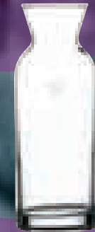
43804 VILLAGE KARAF CARAFFE v:~360 cc. 12 US oz. 12 3/4 UK oz. G*: "none" cc. h: 172 mm. 6 3/4" t: 51 mm. 2" b: 63 mm. 2 1/2" d: 63 mm. 2 1/2" SKU / PACKING 1052702* dk12-0/ob12-0
